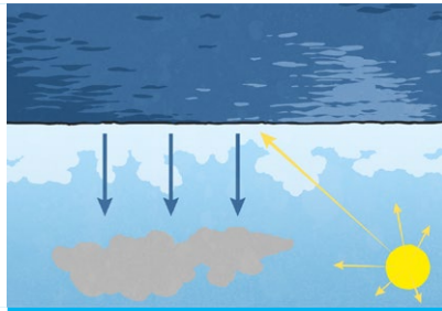
Evaporation
