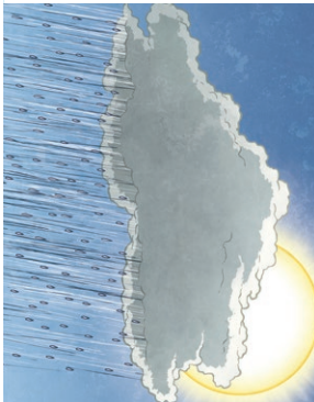
Precipitation
