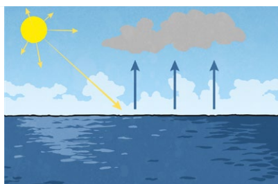
Evaporation
