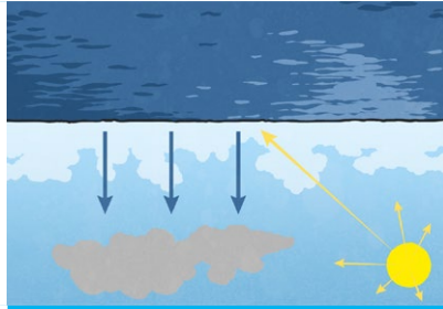
Evaporation
