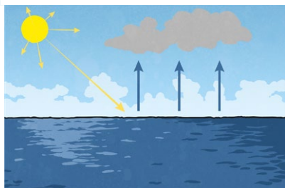
Evaporation
